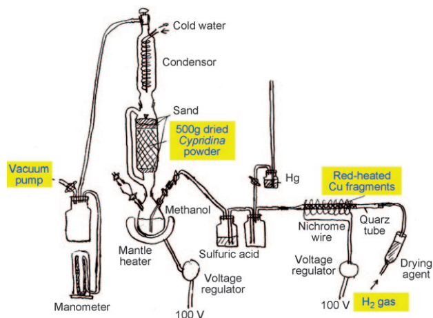
Figure 6. The apparatus used for extracting Cypridina luciferin.
