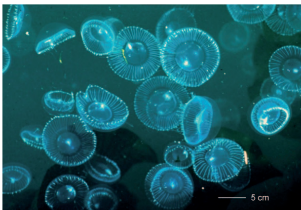
Figure 9. The jellyfish Aequorea aequorea in nature.
