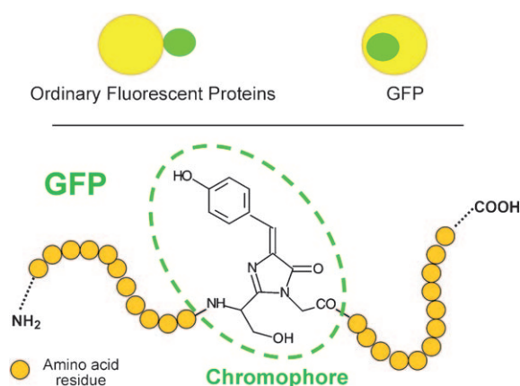
Figure 19. The structure of the chromophore in the molecules of GFP.
