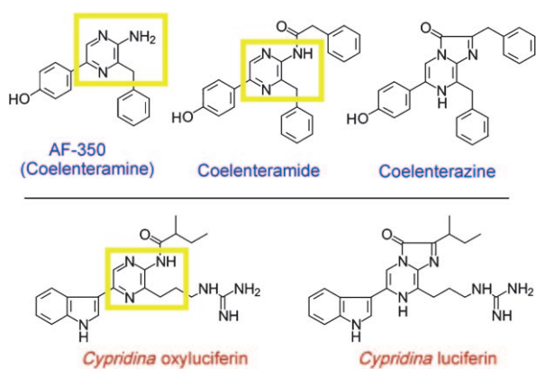
Figure 16. The chemical structures of AF-350 (coelenteramine), coelenteramide (a product of the luminescence reaction of aequorin), and coelenterazine, compared with those of Cypridina oxyluciferin and luciferin.
