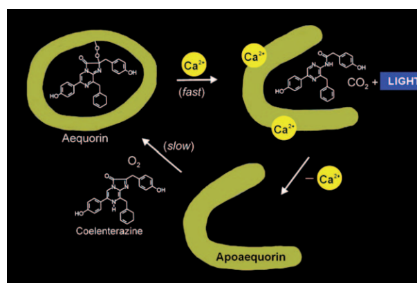
Figure 17. The luminescence and regeneration of aequorin. The photo-protein aequorin binds with two \text{Ca}^{2+} ions, [17,18] and decomposes into coelenteramide, \text{CO}_2 , and apoaequorin accompanied by the emission of light (emission maximum at 465 nm). Apoaequorin can be regenerated into the original aequorin by incubation with coelenterazine in the presence of oxygen.
