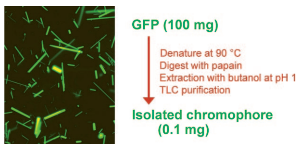
Figure 18. Left: Crystals of GFP (photo by Dr. Shinya Inoué); right: the process of isolating the chromophore of GFP.
