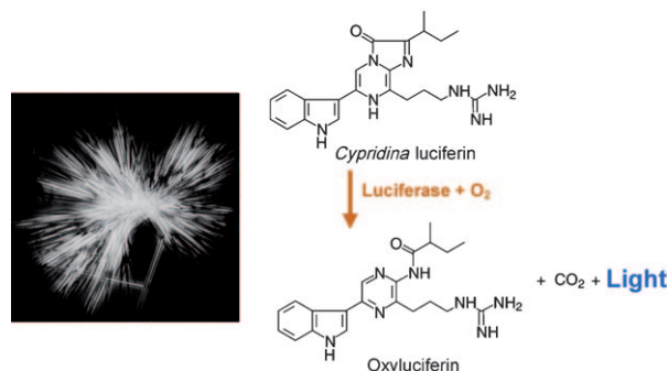
Figure 7. Crystals of Cypridina luciferin (left), and the chemical structures of Cypridina luciferin and its luminescence reaction product, oxyluciferin (right).
